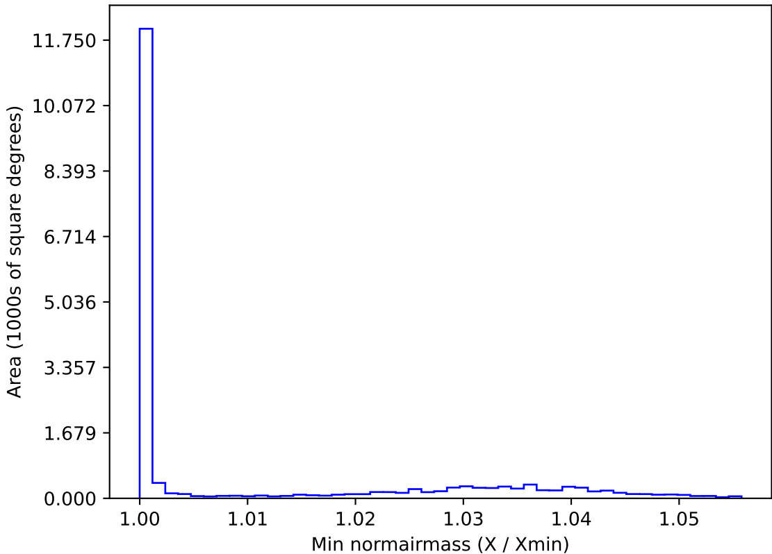
weather_cloudso12v3.4_10yrs WFD u band: Min normairmass
