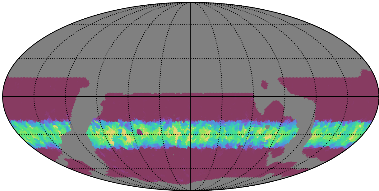
weather_cloudso12v3.4_10yrs WFD g band: Min normairmass
