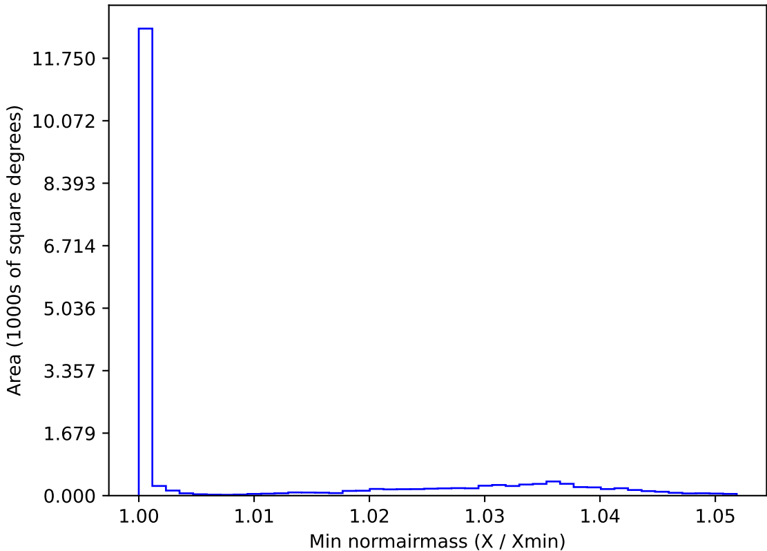
weather_cloudso12v3.4_10yrs WFD g band: Min normairmass
