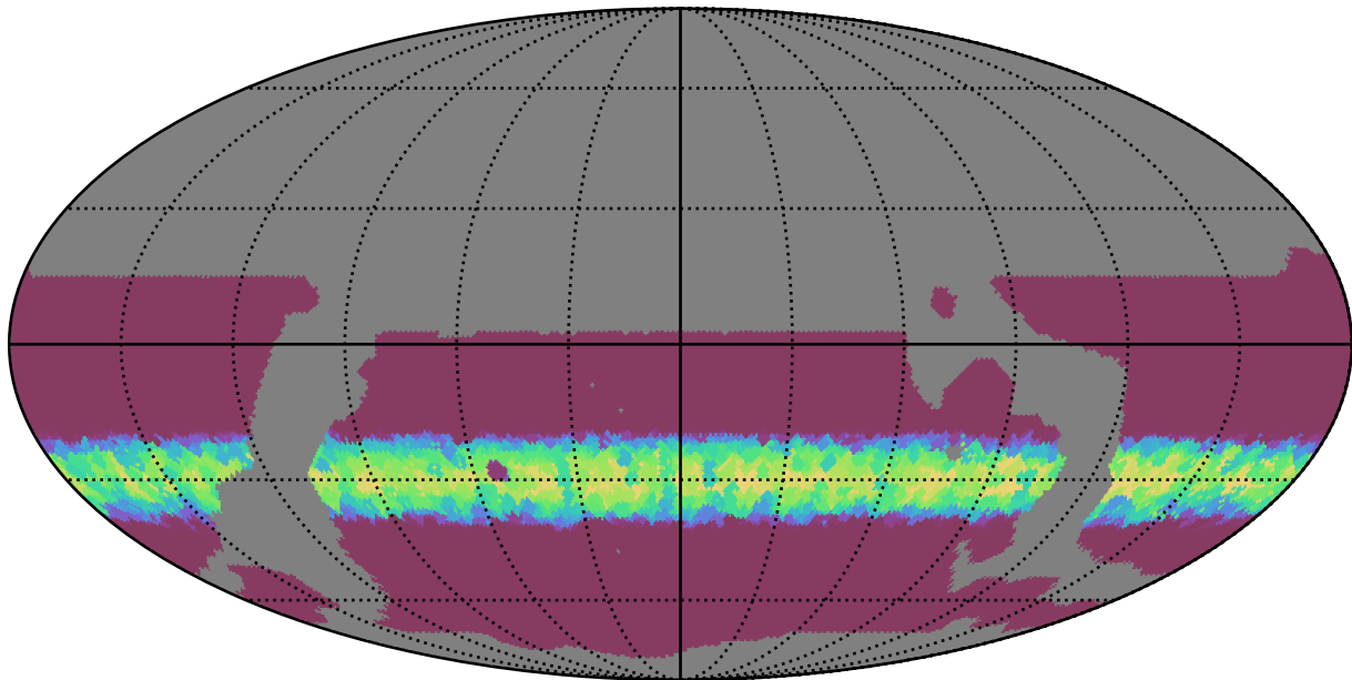
weather_cloudso12v3.4_10yrs WFD all bands: Min normairmass
