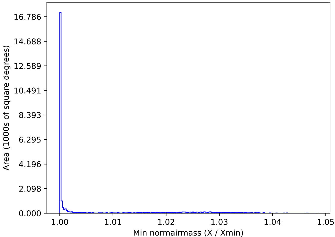
weather_cloudso12v3.4_10yrs All sky z band: Min normairmass
