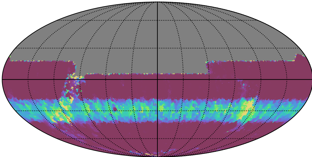
weather_cloudso12v3.4_10yrs All sky u band: Min normairmass
