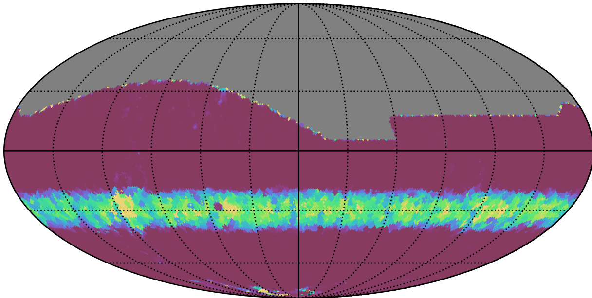
weather_cloudso12v3.4_10yrs All sky r band: Min normairmass
