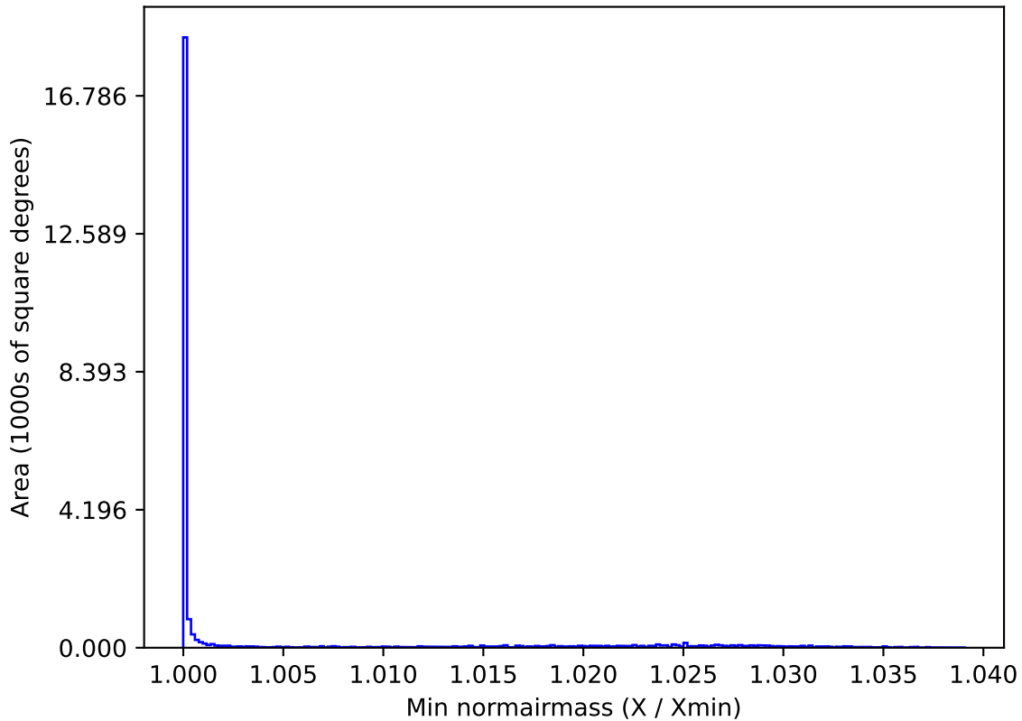
weather_cloudso12v3.4_10yrs All sky i band: Min normairmass
