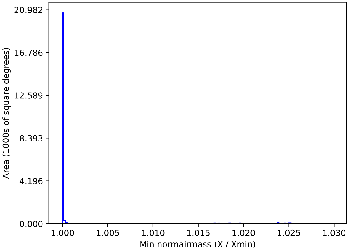
weather_cloudso12v3.4_10yrs All sky all bands: Min normairmass
