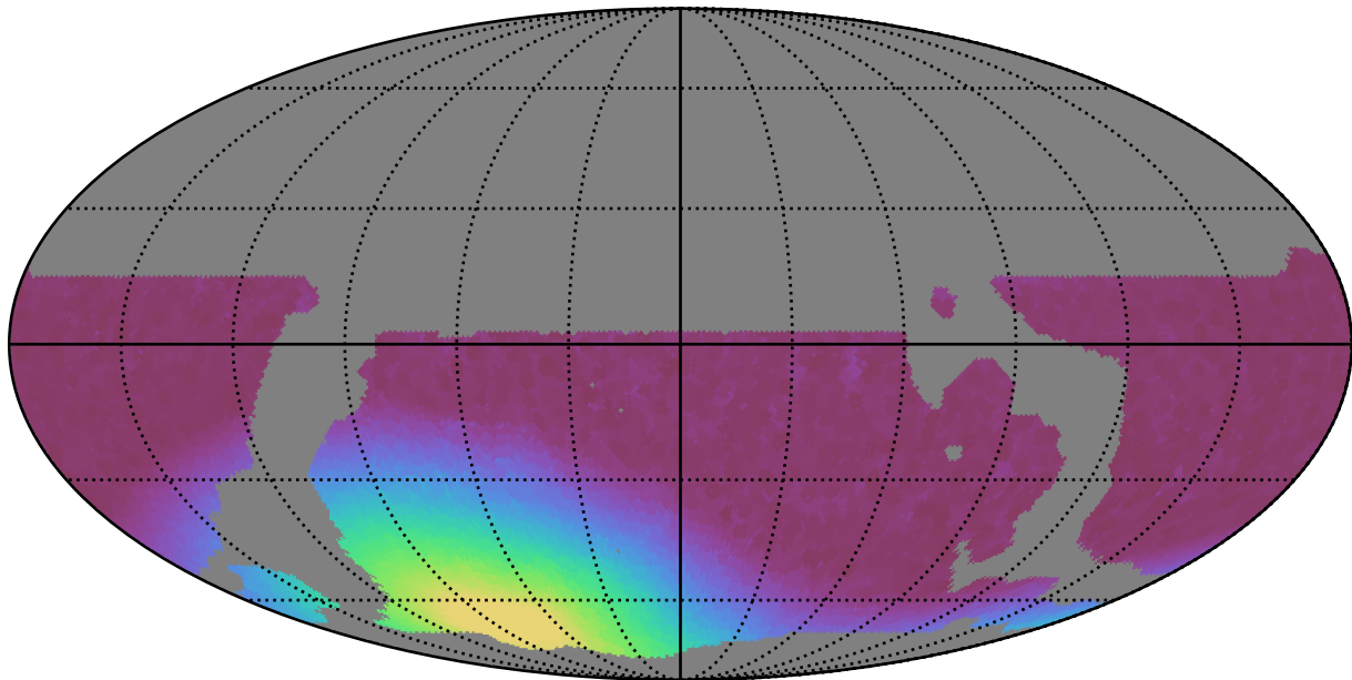
weather_cloudso12v3.4_10yrs WFD z band: Min moonDistance
