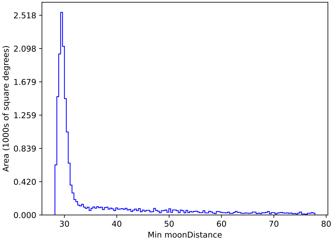
weather_cloudso12v3.4_10yrs WFD z band: Min moonDistance
