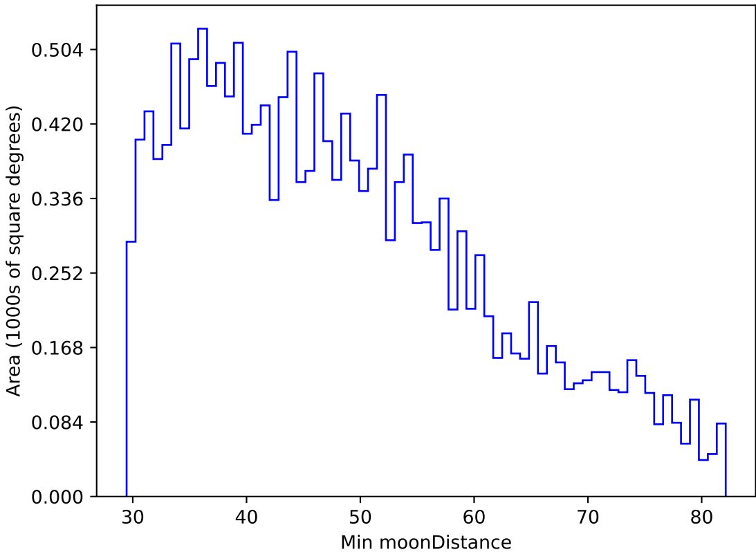
weather_cloudso12v3.4_10yrs WFD u band: Min moonDistance
