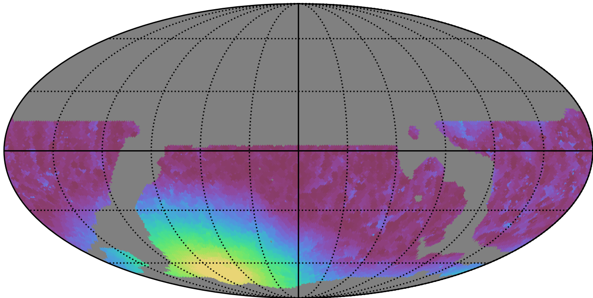
weather_cloudso12v3.4_10yrs WFD r band: Min moonDistance
