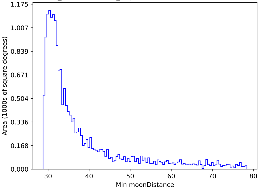
weather_cloudso12v3.4_10yrs WFD r band: Min moonDistance
