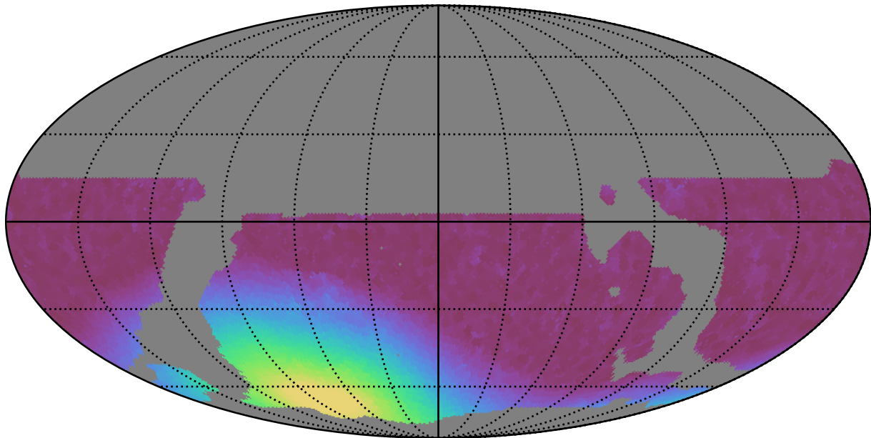
weather_cloudso12v3.4_10yrs WFD i band: Min moonDistance
