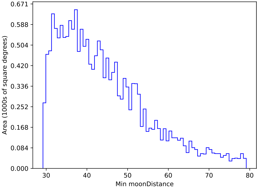
weather_cloudso12v3.4_10yrs WFD g band: Min moonDistance
