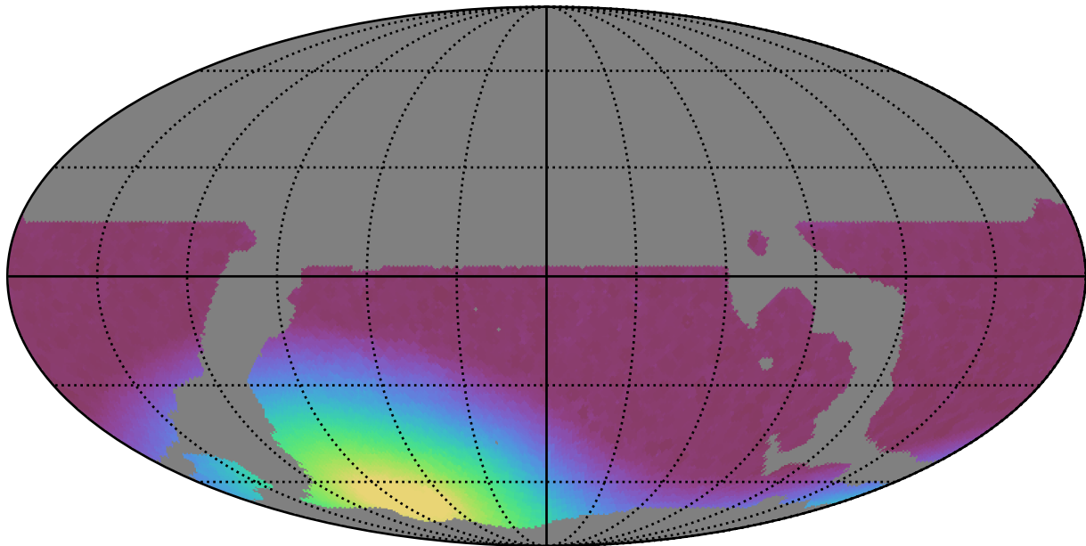
weather_cloudso12v3.4_10yrs WFD all bands: Min moonDistance
