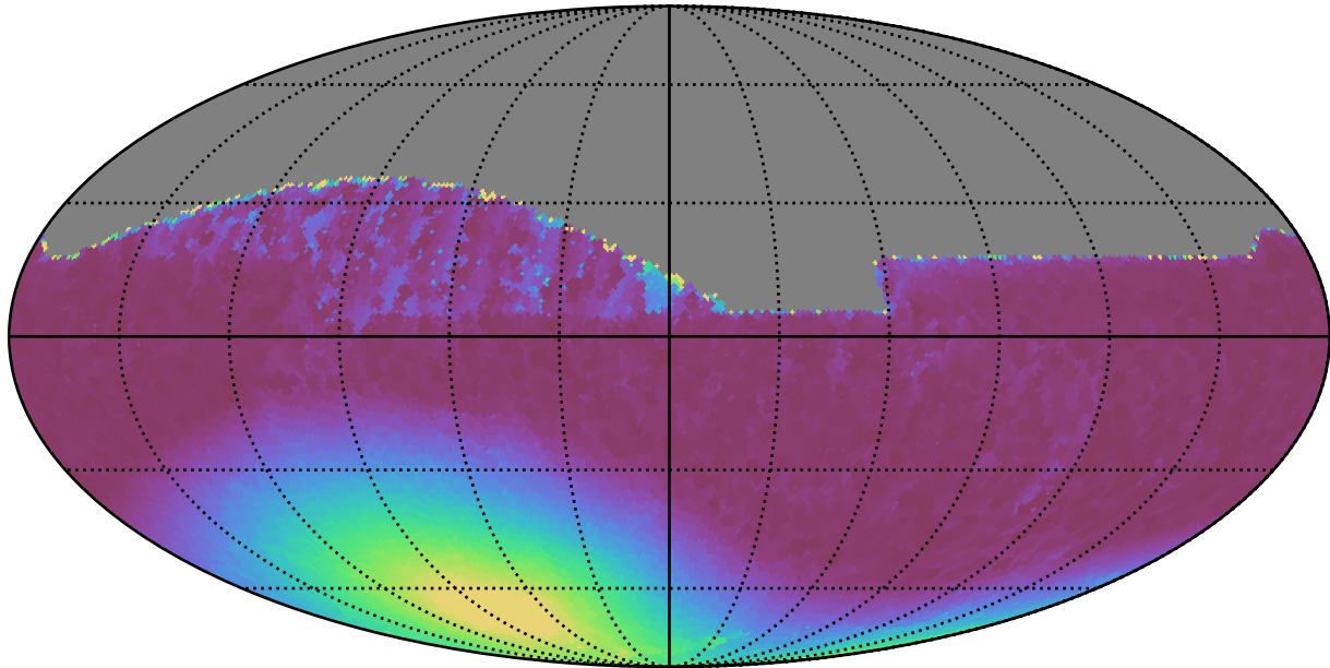
weather_cloudso12v3.4_10yrs All sky z band: Min moonDistance
