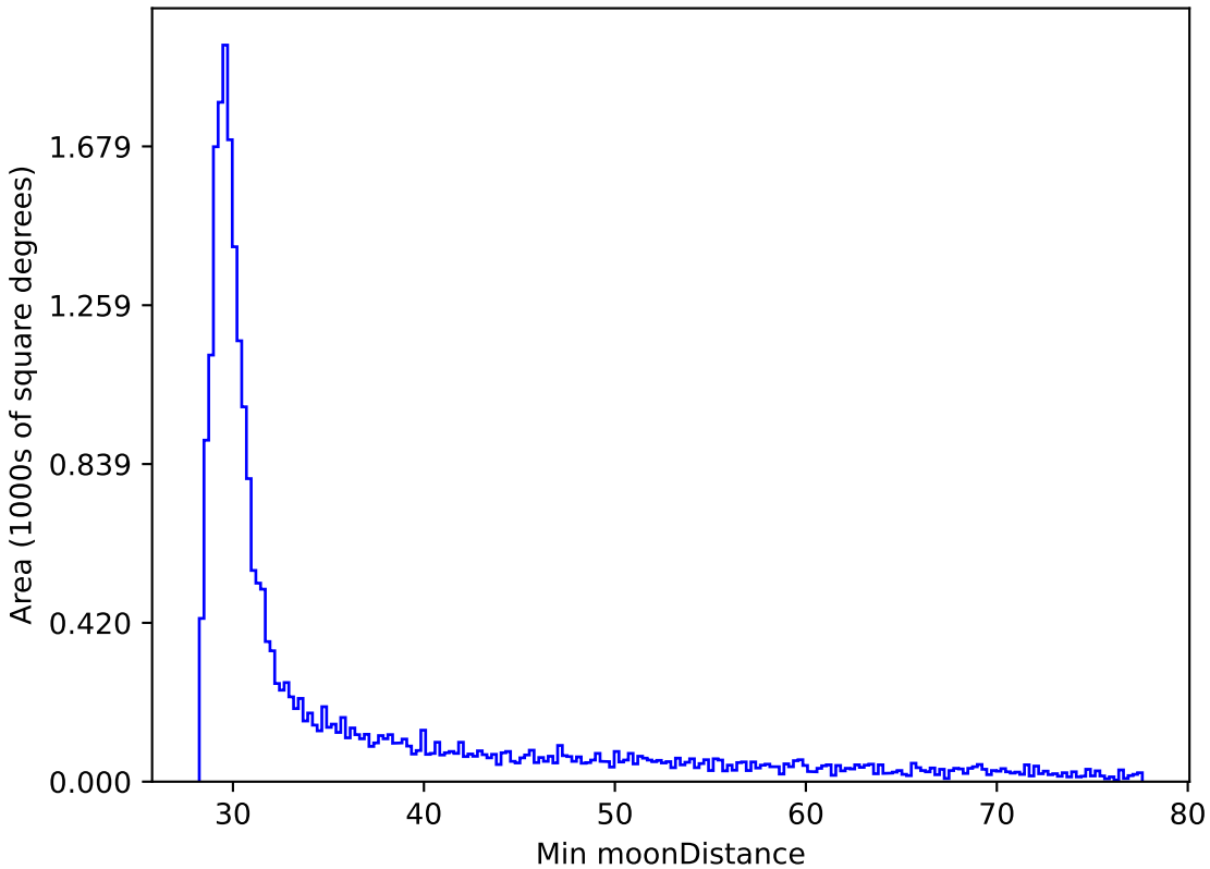
weather_cloudso12v3.4_10yrs All sky z band: Min moonDistance
