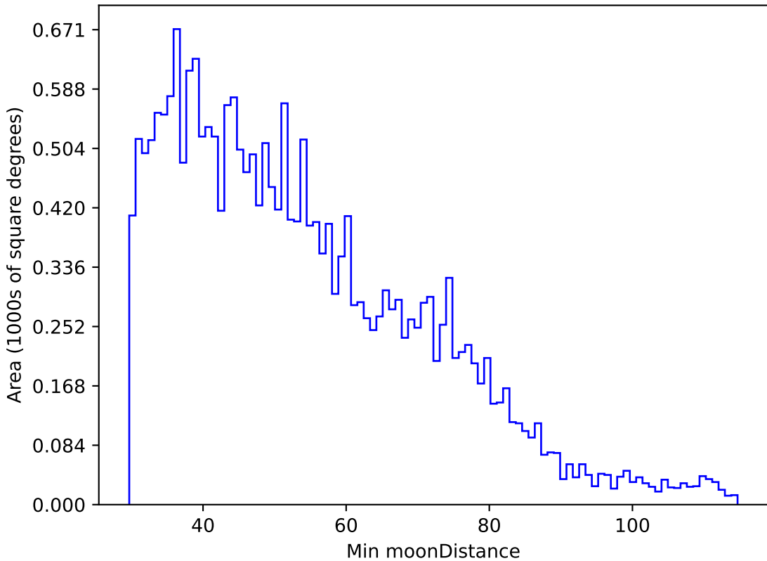
weather_cloudso12v3.4_10yrs All sky u band: Min moonDistance
