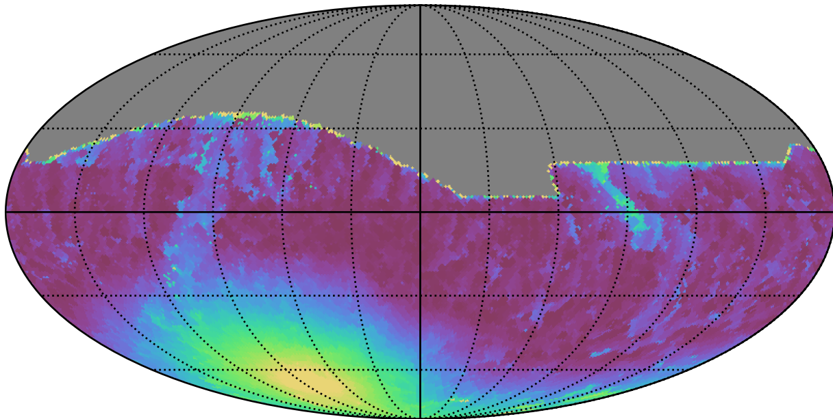
weather_cloudso12v3.4_10yrs All sky r band: Min moonDistance
