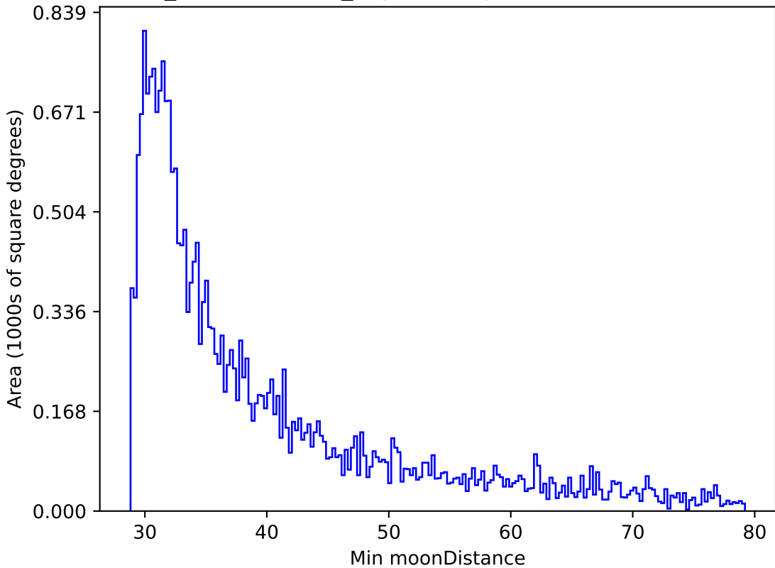
weather_cloudso12v3.4_10yrs All sky r band: Min moonDistance
