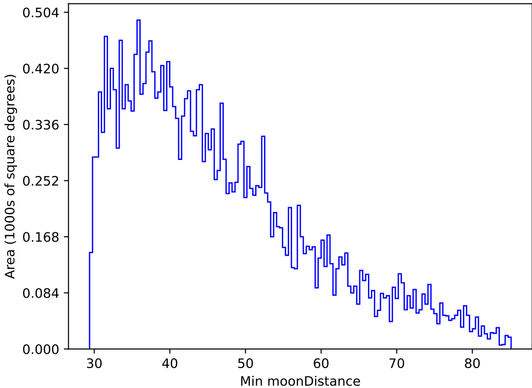
weather_cloudso12v3.4_10yrs All sky g band: Min moonDistance
