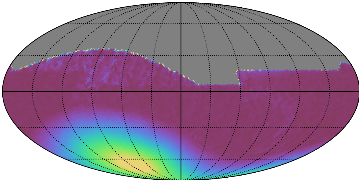
weather_cloudso12v3.4_10yrs All sky all bands: Min moonDistance
