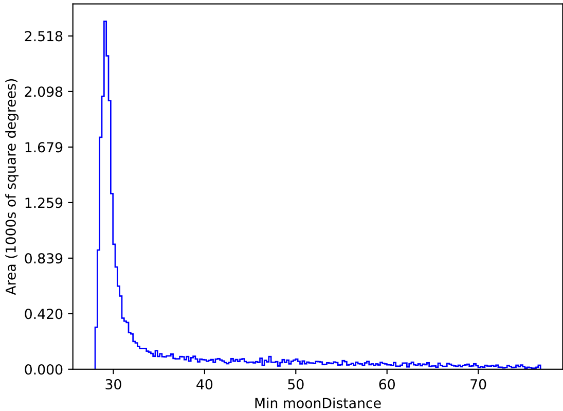
weather_cloudso12v3.4_10yrs All sky all bands: Min moonDistance
