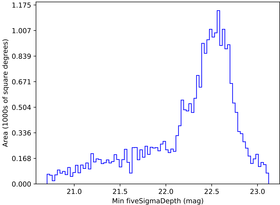
weather_cloudso12v3.4_10yrs Yr 1 z band: Min fiveSigmaDepth
