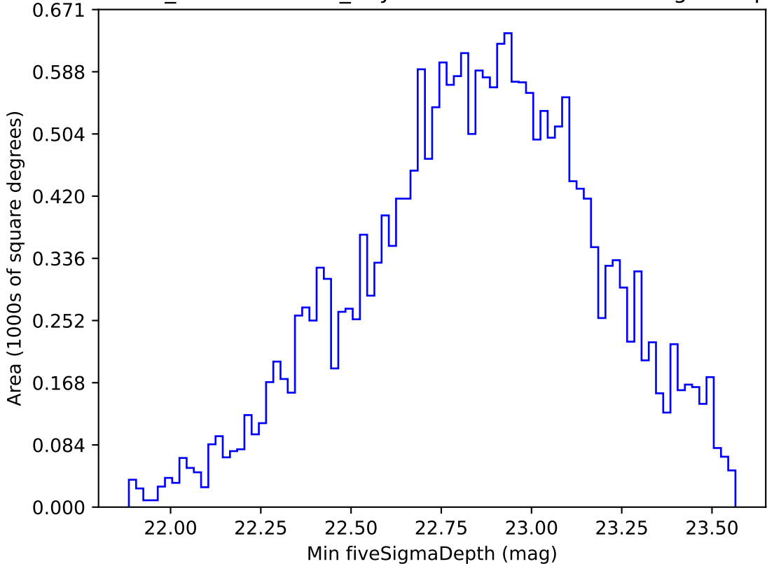
weather_cloudso12v3.4_10yrs Yr 1 u band: Min fiveSigmaDepth
