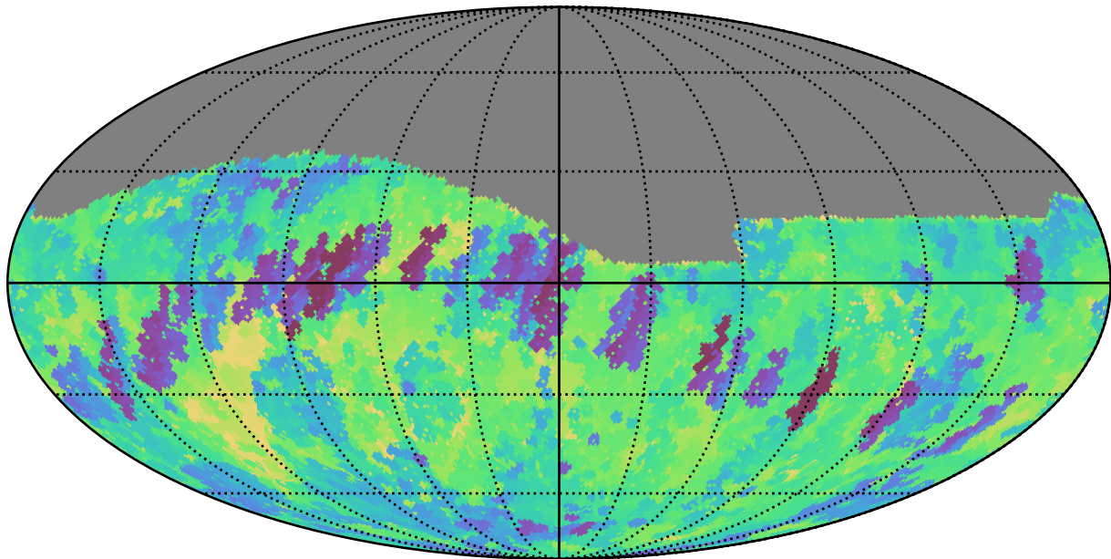
weather_cloudso12v3.4_10yrs Yr 1 r band: Min fiveSigmaDepth
