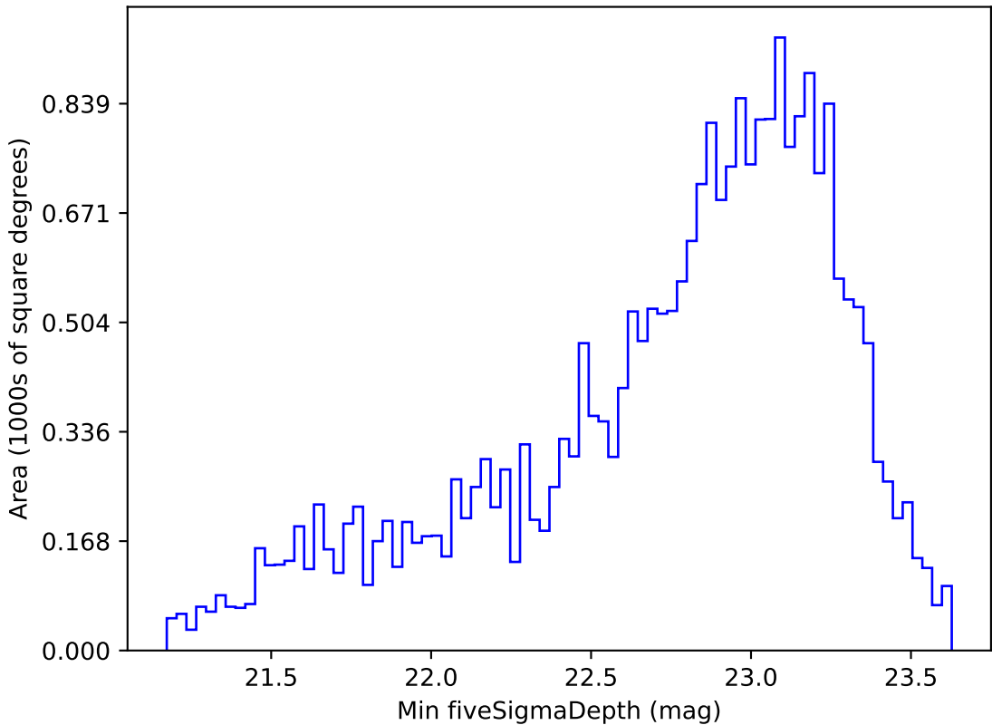
weather_cloudso12v3.4_10yrs Yr 1 i band: Min fiveSigmaDepth
