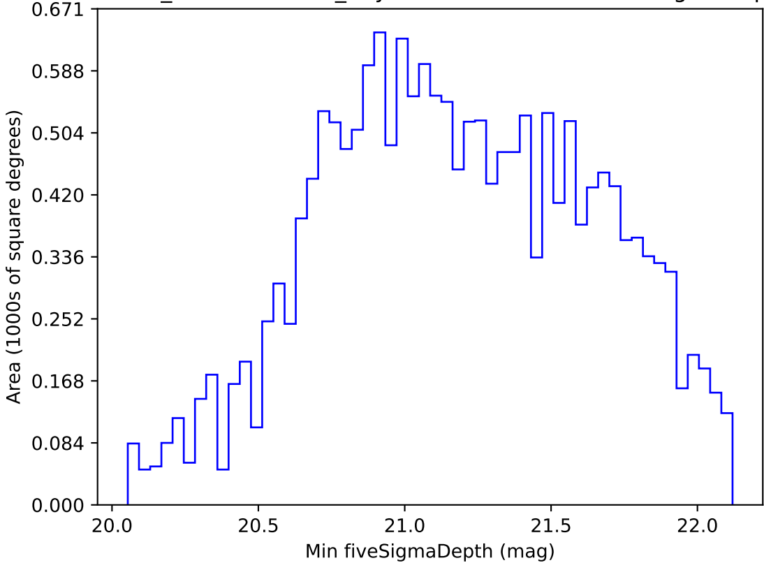
weather_cloudso12v3.4_10yrs WFD z band: Min fiveSigmaDepth
