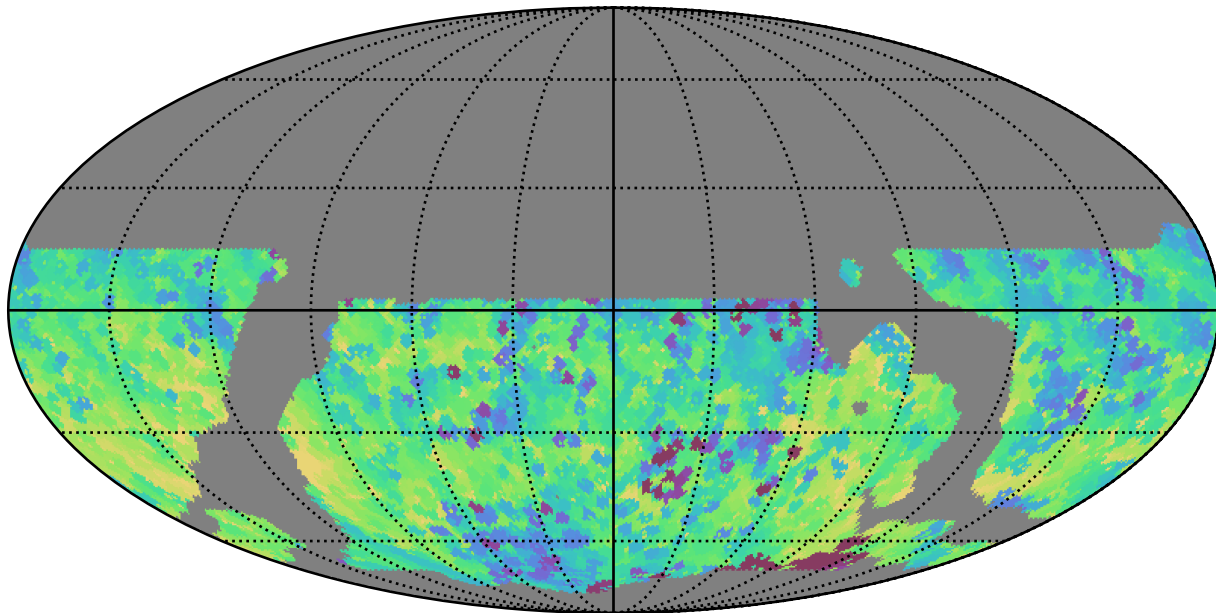
weather_cloudso12v3.4_10yrs WFD y band: Min fiveSigmaDepth
