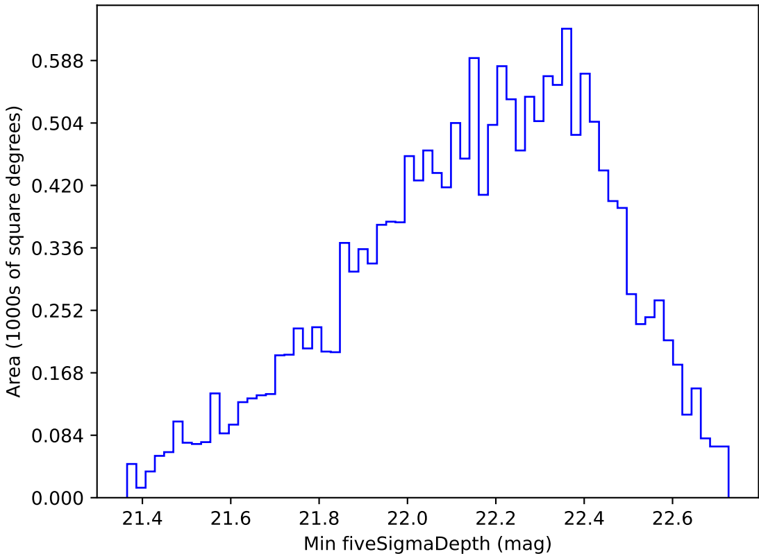
weather_cloudso12v3.4_10yrs WFD u band: Min fiveSigmaDepth
