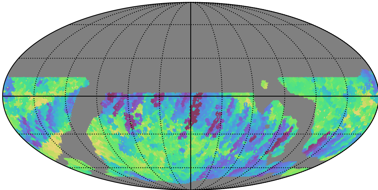
weather_cloudso12v3.4_10yrs WFD r band: Min fiveSigmaDepth
