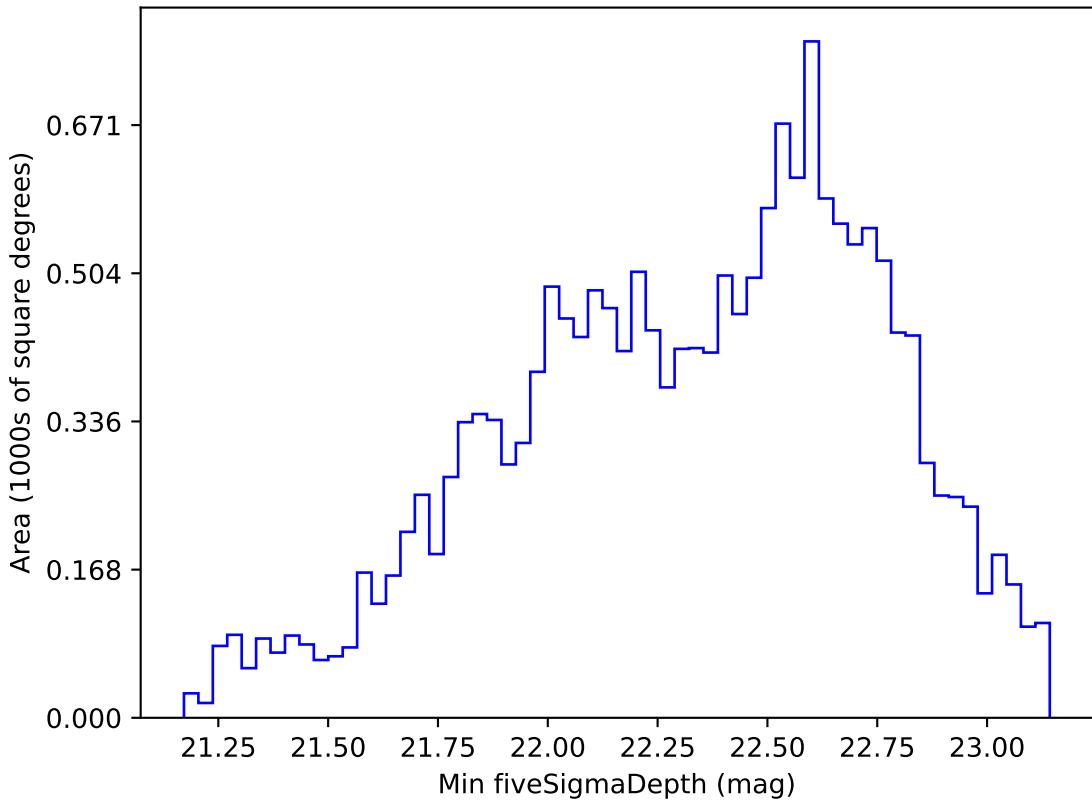
weather_cloudso12v3.4_10yrs WFD r band: Min fiveSigmaDepth
