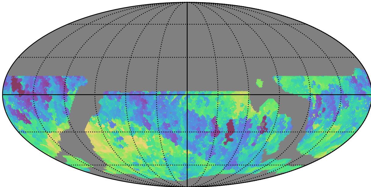
weather_cloudso12v3.4_10yrs WFD i band: Min fiveSigmaDepth
