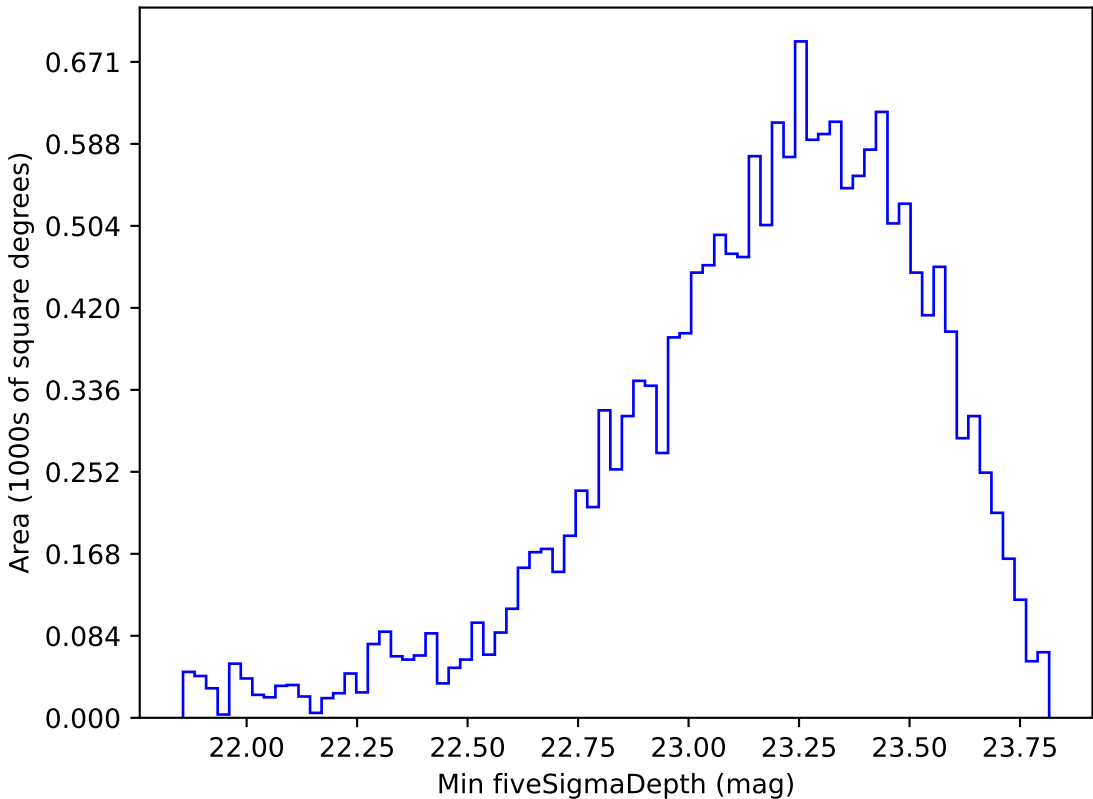
weather_cloudso12v3.4_10yrs WFD g band: Min fiveSigmaDepth
