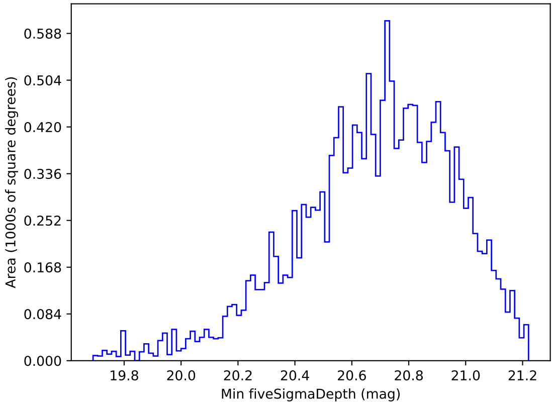
weather_cloudso12v3.4_10yrs WFD all bands: Min fiveSigmaDepth
