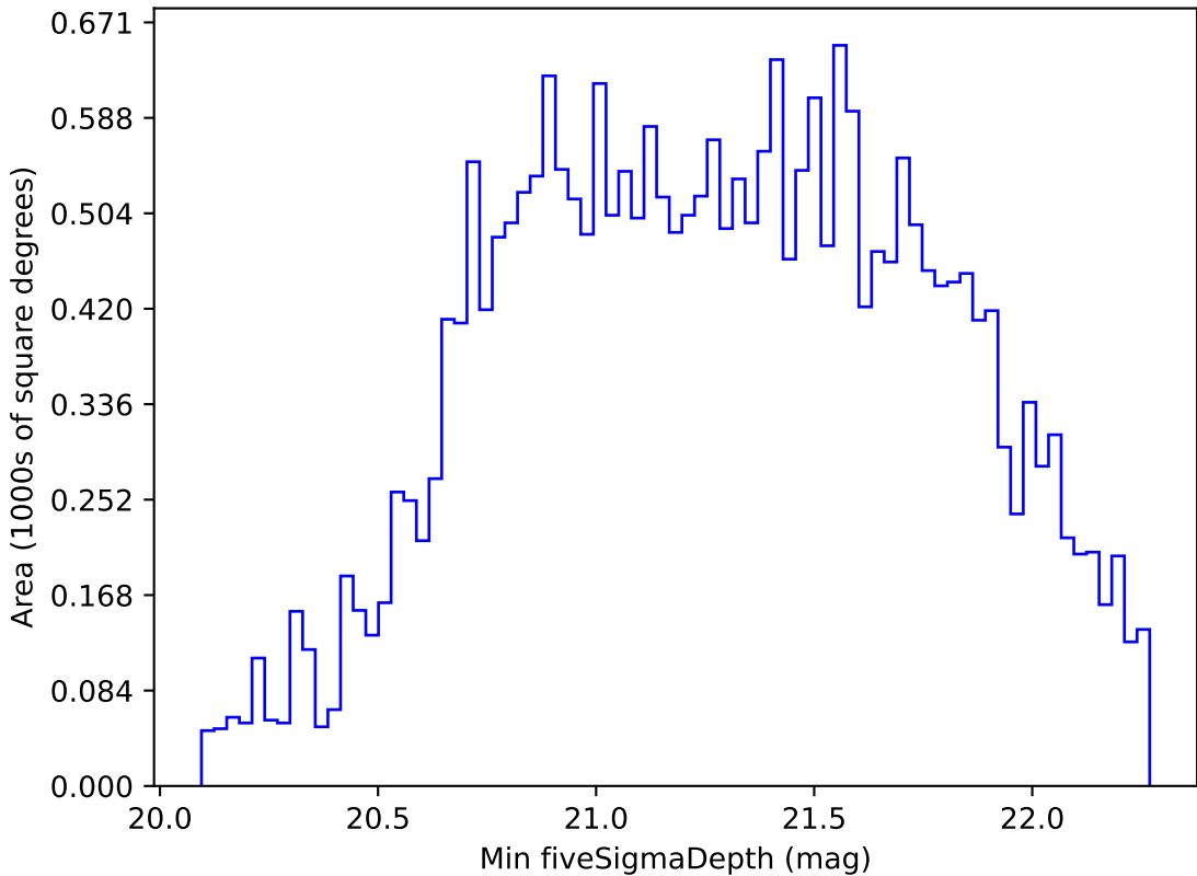
weather_cloudso12v3.4_10yrs All sky z band: Min fiveSigmaDepth
