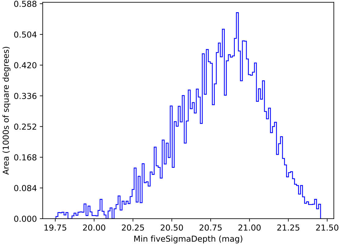
weather_cloudso12v3.4_10yrs All sky y band: Min fiveSigmaDepth
