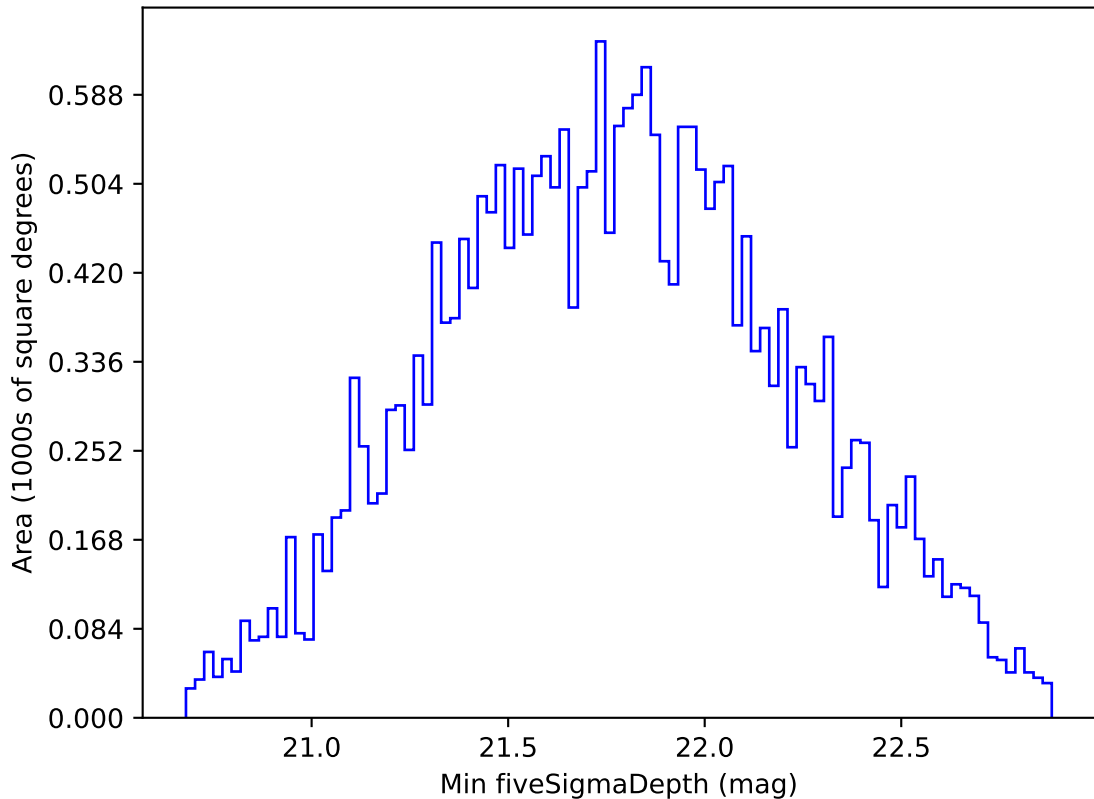
weather_cloudso12v3.4_10yrs All sky i band: Min fiveSigmaDepth
