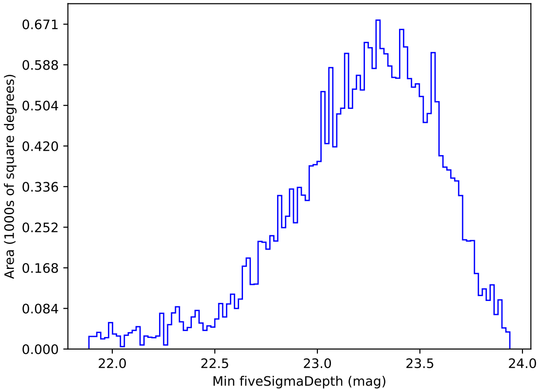
weather_cloudso12v3.4_10yrs All sky g band: Min fiveSigmaDepth
