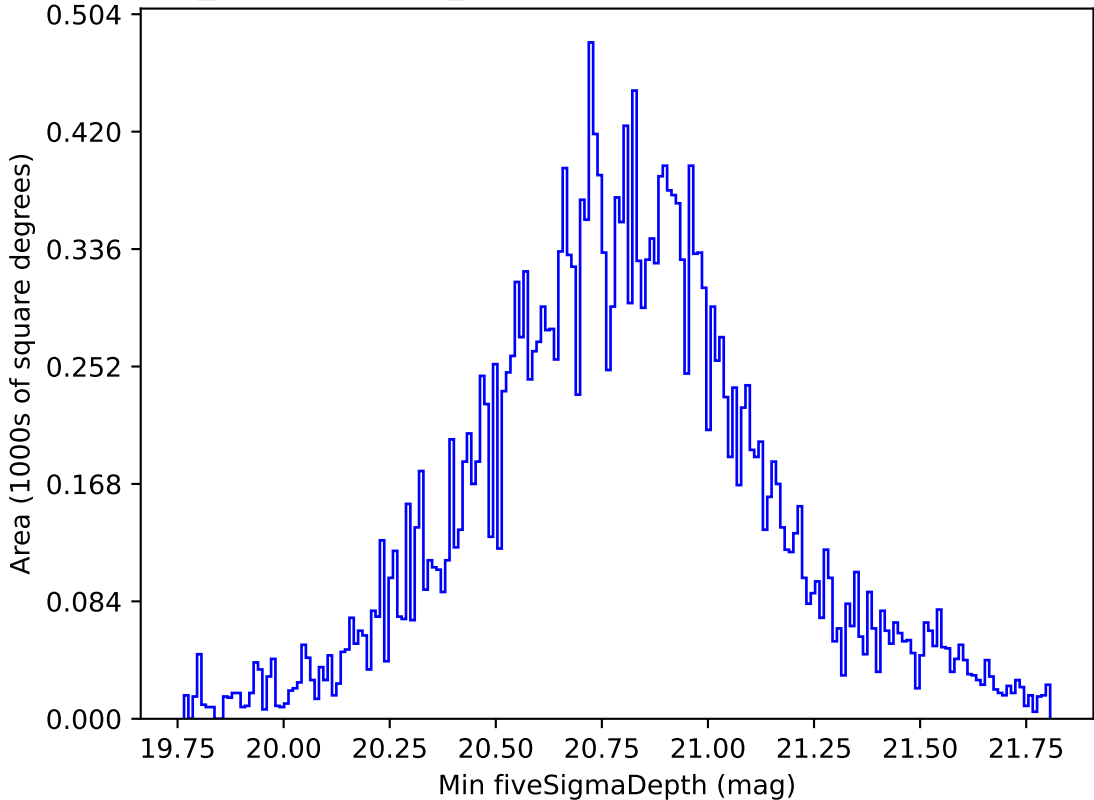
weather_cloudso12v3.4_10yrs All sky all bands: Min fiveSigmaDepth
