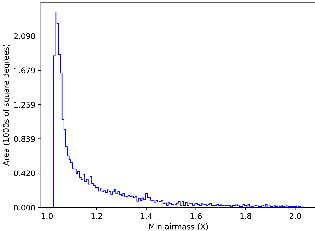
weather_cloudso12v3.4_10yrs Yr 1 z band: Min airmass
