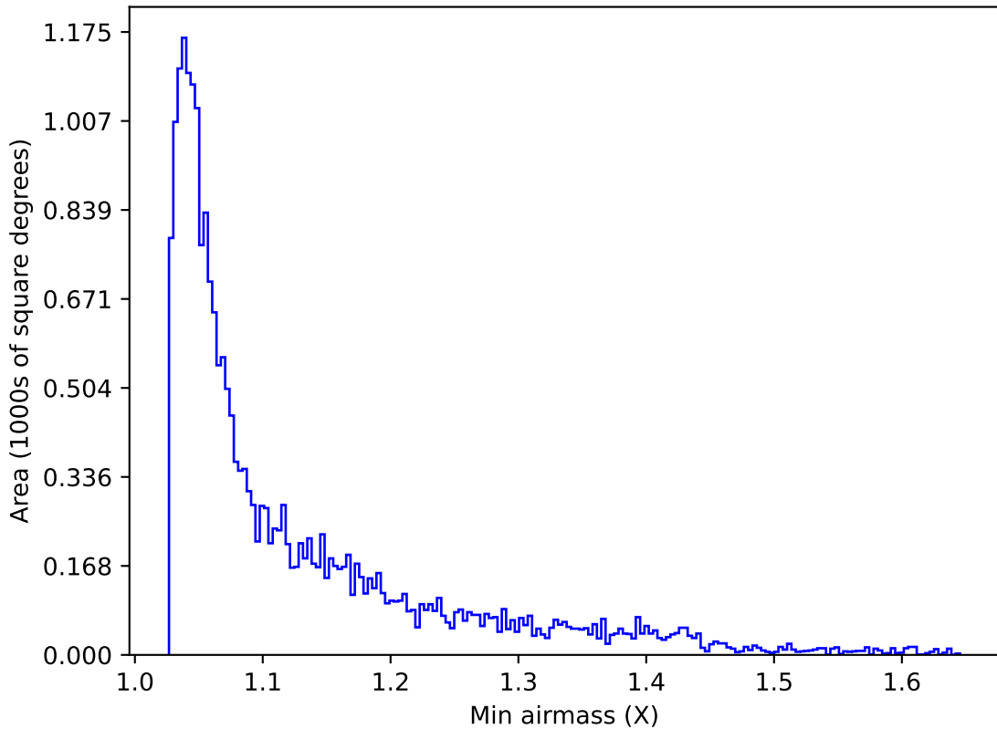
weather_cloudso12v3.4_10yrs Yr 1 y band: Min airmass
