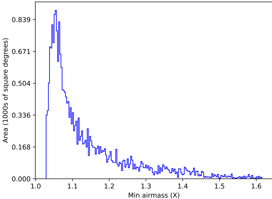
weather_cloudso12v3.4_10yrs Yr 1 u band: Min airmass
