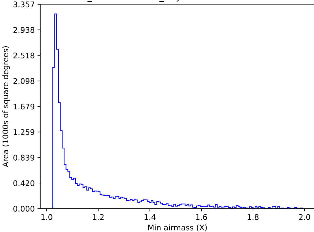
weather_cloudso12v3.4_10yrs Yr 1 r band: Min airmass
