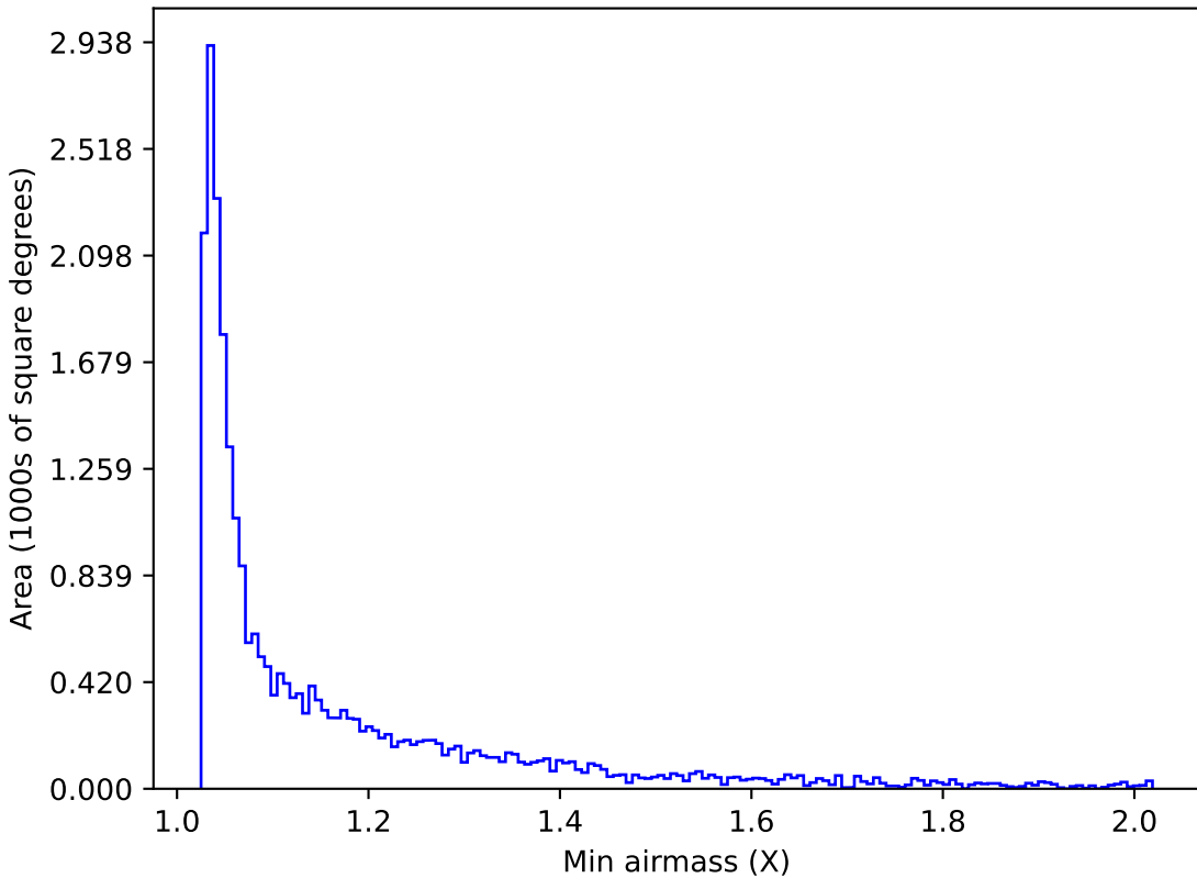
weather_cloudso12v3.4_10yrs Yr 1 i band: Min airmass
