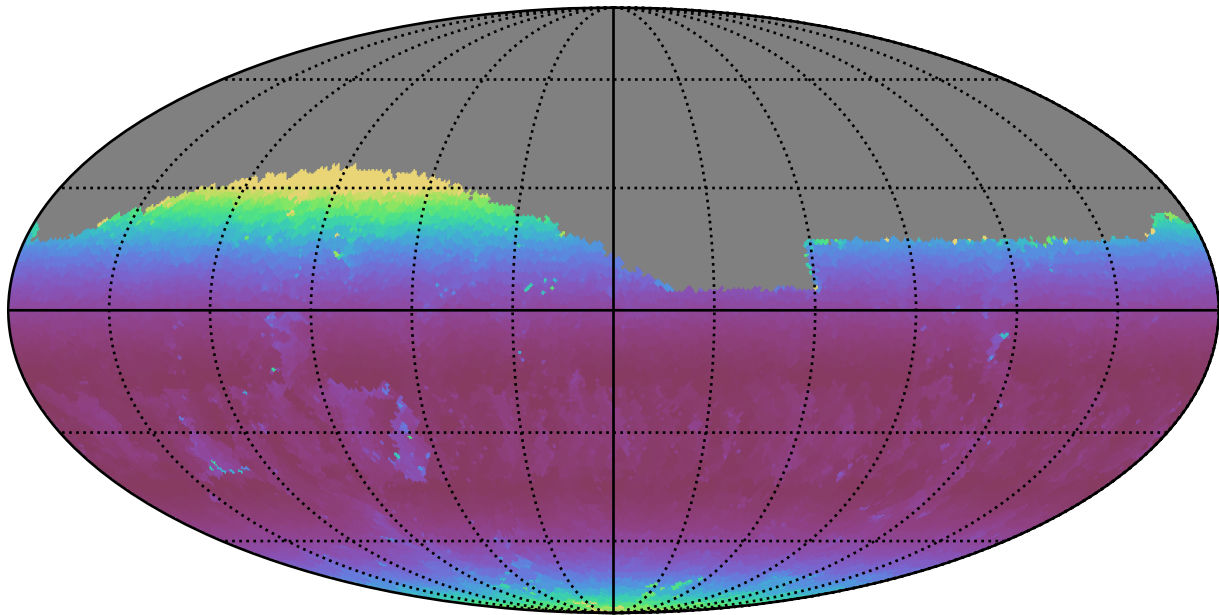
weather_cloudso12v3.4_10yrs Yr 1 g band: Min airmass
