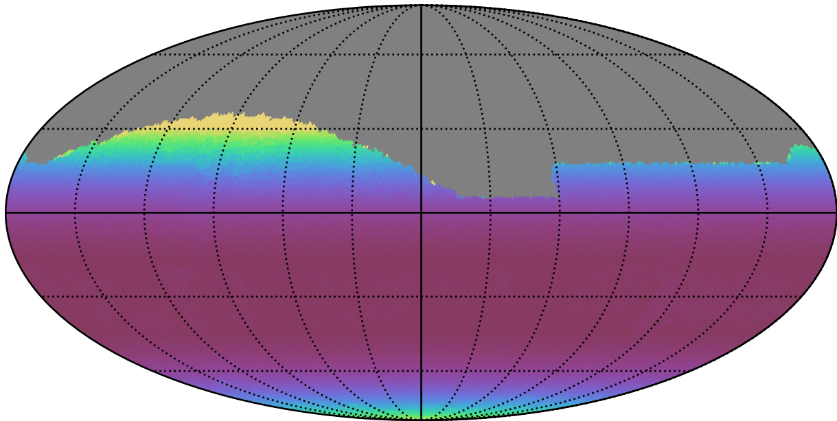
weather_cloudso12v3.4_10yrs Yr 1 all bands: Min airmass
