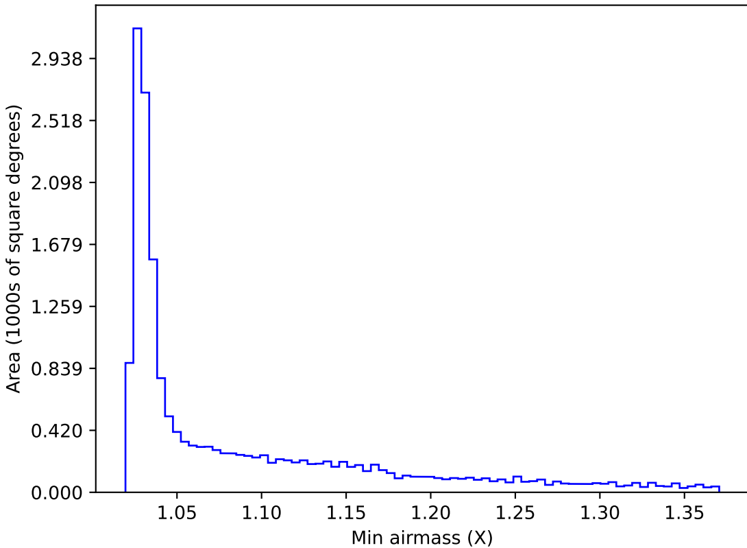
weather_cloudso12v3.4_10yrs WFD z band: Min airmass
